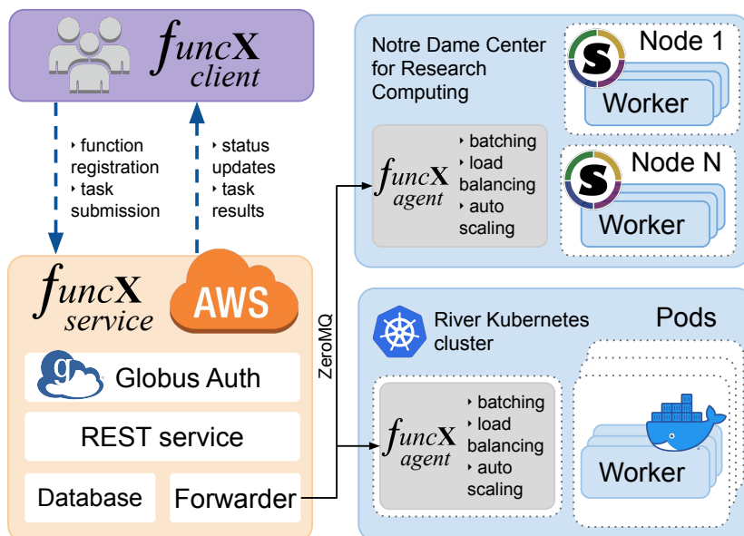
Figure 1. Overview of the funcX system architecture. The The funcX client abstracts interactions with funcX. The funcX service is used to register and manage endpoints, register and execute functions, and retrieve results. FuncX endpoints are deployed on remote computers (in this case at Notre Dame and the River Kubernetes cluster) and enable function execution on provisioned nodes, optionally using locally supported containers.
